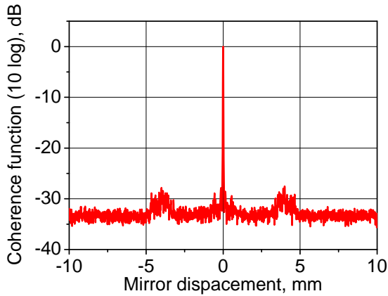
Coherence function at 5 mW power level (extended displacement)
