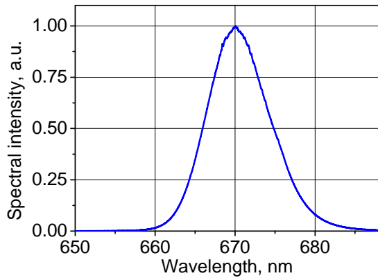
Spectrum at 5 mW power level
