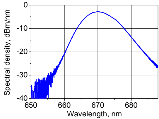
Spectral density at 5 mW power level
