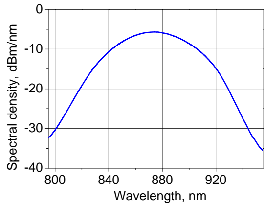
Spectral density at 15 mW power level
