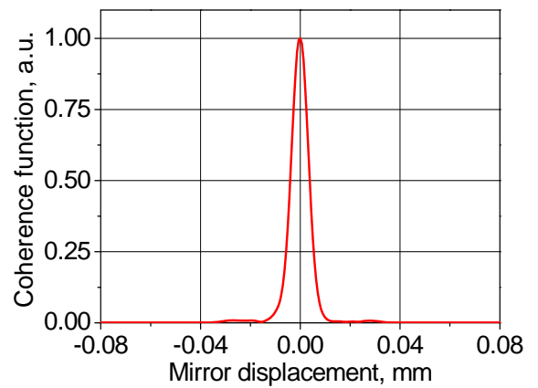
Coherence function at 15 mW power level (short displacement)
