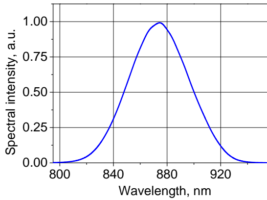
Spectrum at 15 mW power level
