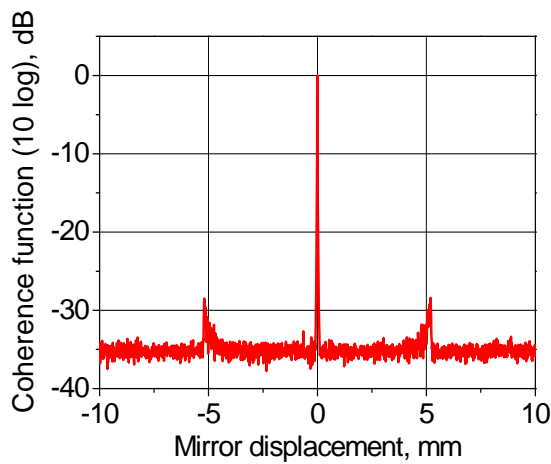
Coherence function at 15 mW power level (extended displacement)
