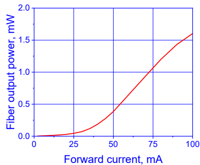
Light-current curve
