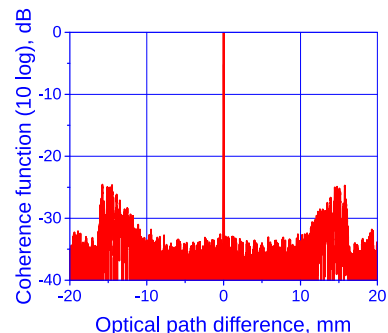
Coherence at rated power
