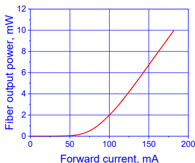
Light-current curve
