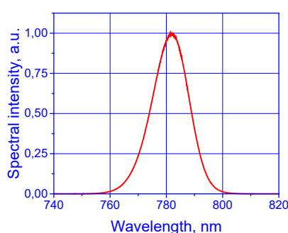
Spectrum at rated power
