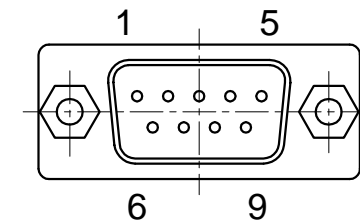
View A (2/1)
